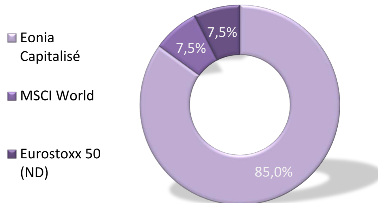
Composition Benchmark
